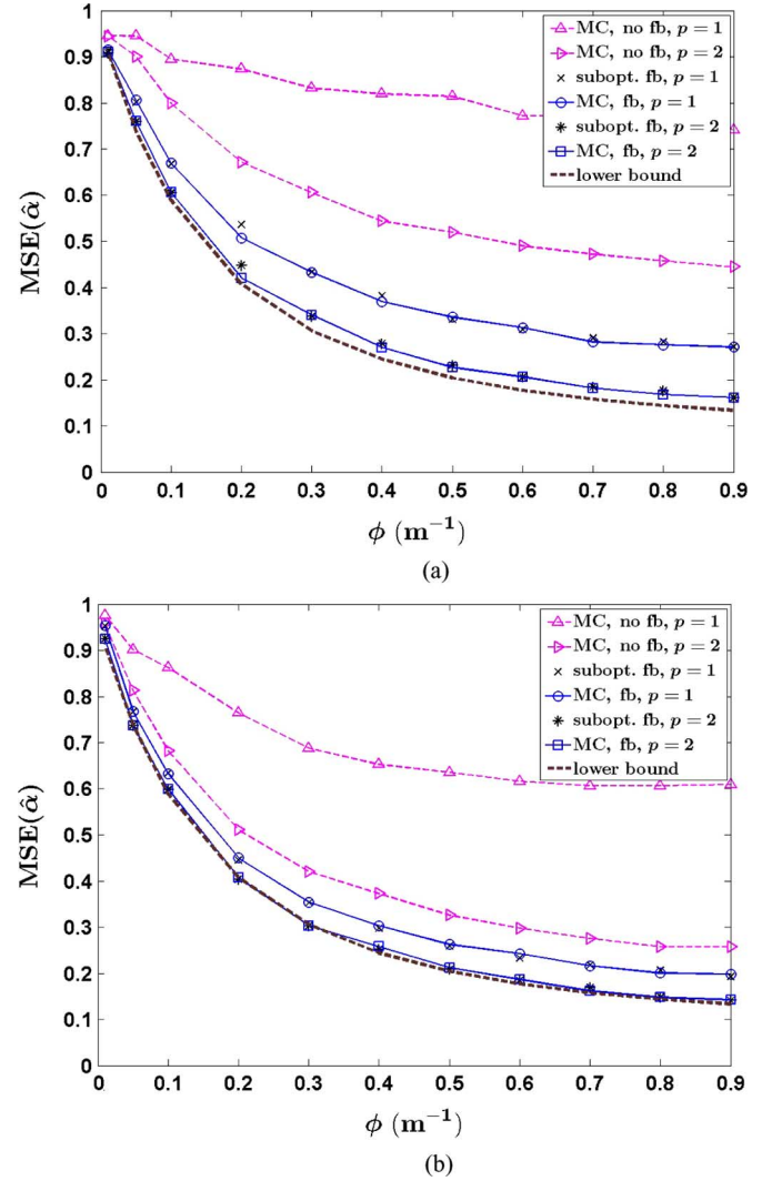
Fig. 3. Constant mean-signal scenario: Average MSEs of various estimators of \alpha as functions of \phi , for (a) K = 2 and (b) K = 3 quantization intervals and p \in \{1, 2\} rounds.
