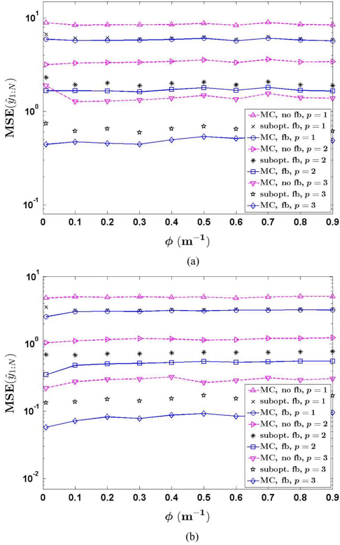
Fig. 9. Linear trend-surface scenario: Average MSEs of the proposed estimators of \mathbf{y}_{1:N} as functions of \phi , for (a) K = 2 and (b) K = 3 quantization intervals and p \in \{1, 2, 3\} rounds.
