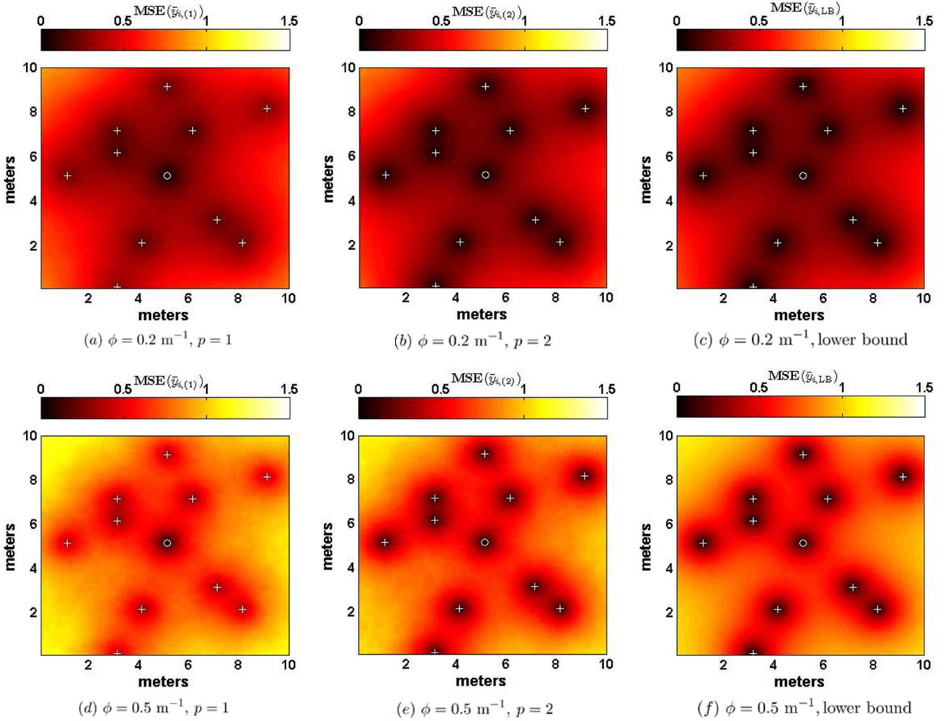
Fig. 6. Constant mean-signal scenario: average MSEs of the feedback MC random-field predictors for (a) \phi = 0.2 \text{ m}^{-1} and p = 1 round, (b) \phi = 0.2 \text{ m}^{-1} and p = 2 rounds, (c) lower bound for \phi = 0.2 \text{ m}^{-1} , (d) \phi = 0.5 \text{ m}^{-1} and p = 1 , (e) \phi = 0.5 \text{ m}^{-1} and p = 2 , and (f) lower bound for \phi = 0.5 \text{ m}^{-1} , using K = 3 quantization intervals.
