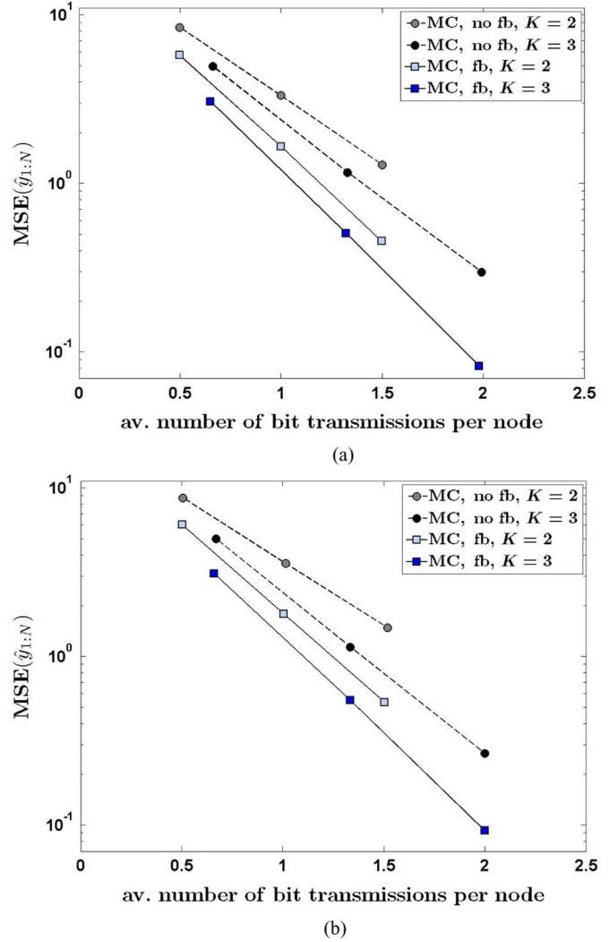
Fig. 10. Linear trend-surface scenario: Average MSEs of MC random-field estimators as functions of the average number of bit transmissions per node, for (a) \phi = 0.2 \text{ m}^{-1} and (b) \phi = 0.5 \text{ m}^{-1} .
