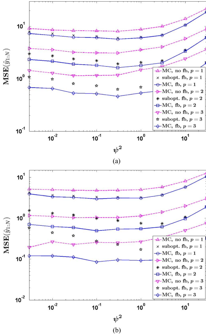
Fig. 13. Linear trend-surface scenario: Average MSEs of the proposed estimators of \mathbf{y}_{1:N} as functions of \psi^2 for (a) K = 2 and (b) K = 3 quantization intervals and p \in \{1, 2, 3\} rounds.
