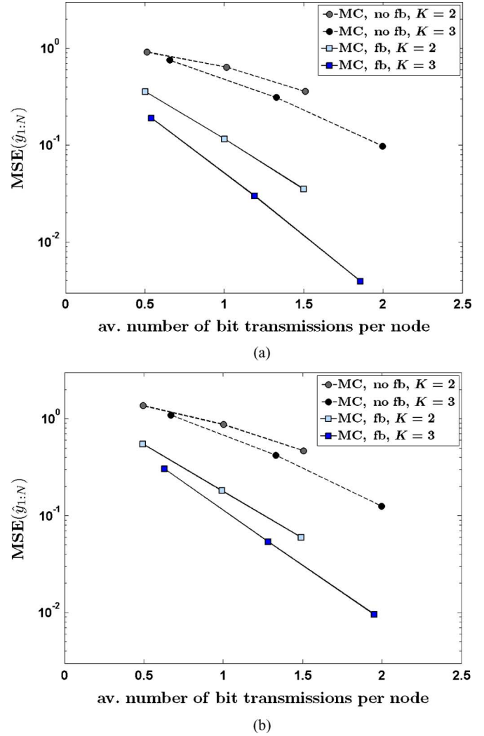
Fig. 5. Constant mean-signal scenario: Average MSEs of MC random-field estimators as functions of the average number of bit transmissions per node, for (a) \phi = 0.2 \text{ m}^{-1} and (b) \phi = 0.5 \text{ m}^{-1} .
