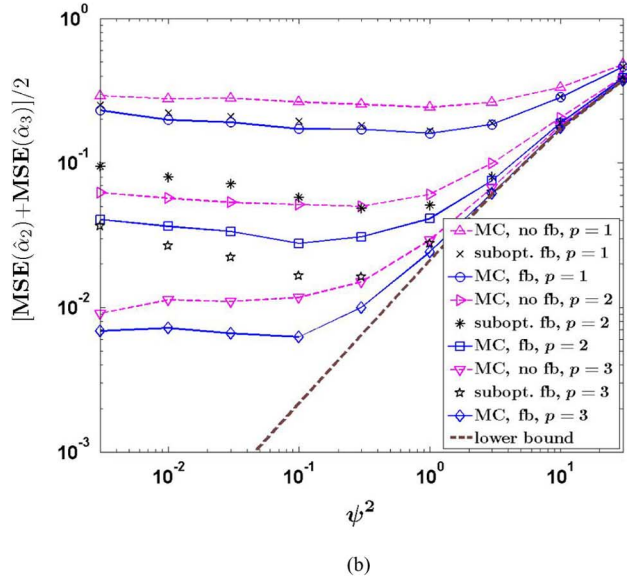
Fig. 12. Linear trend-surface scenario: (a) \text{MSE}(\hat{\alpha}_1) and (b) (1/2)[\text{MSE}(\hat{\alpha}_2) + \text{MSE}(\hat{\alpha}_3)] as functions of \psi^2 , for K = 3 quantization intervals.
