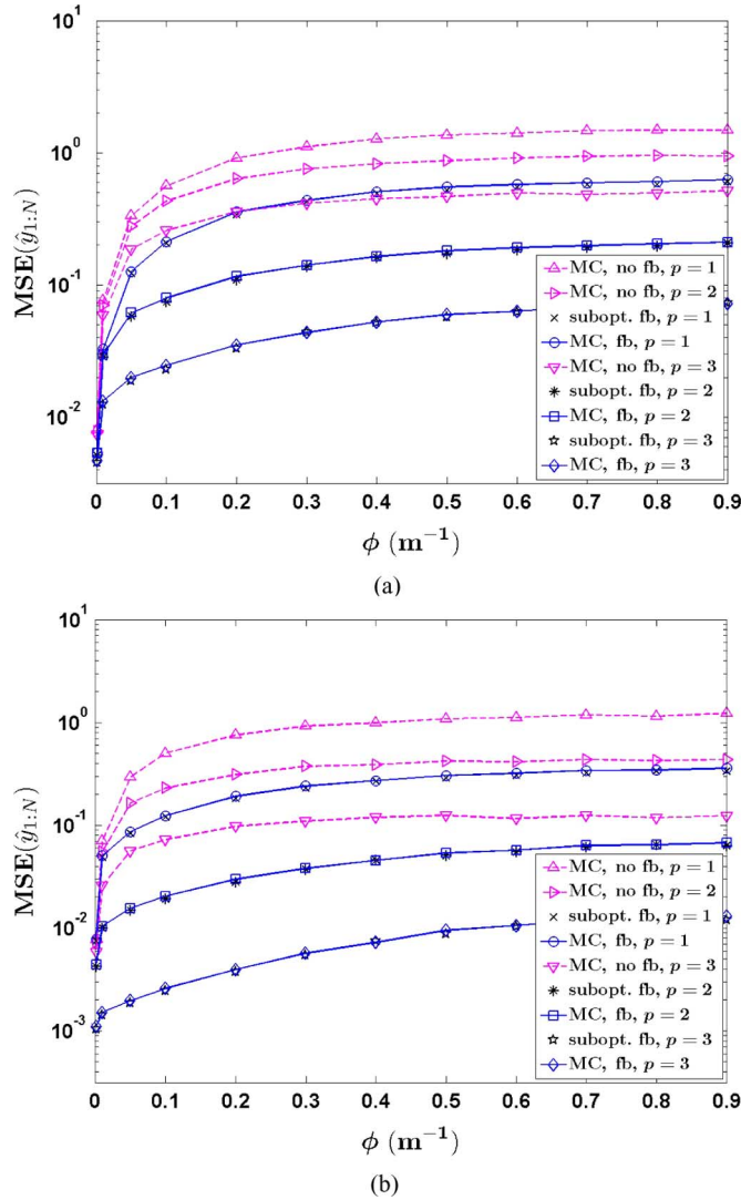
Fig. 4. Constant mean-signal scenario: Average MSEs of various estimators of \mathbf{y}_{1:N} as functions of \phi , for (a) K = 2 and (b) K = 3 quantization intervals and p \in \{1, 2, 3\} rounds.
