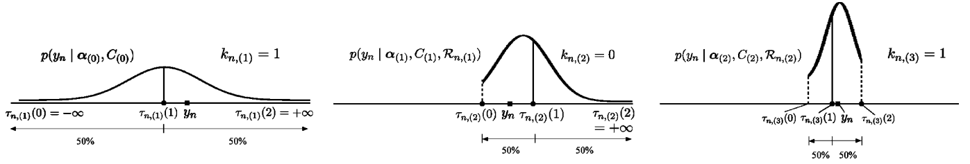
Fig. 1. Rounds 1, 2, and 3 of the proposed adaptive quantization scheme, for K = 2 quantization intervals.
